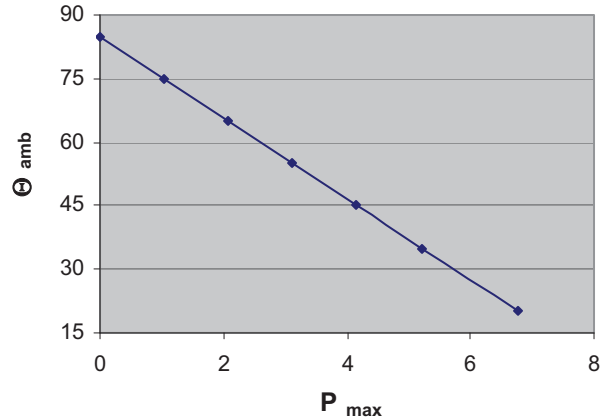
Max. allowable ambient Temp. at specific power loss B25673A0102A400
