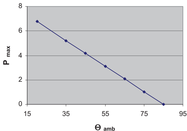
Max. allowable power loss at specific ambient Temp. B25673A0102A400
