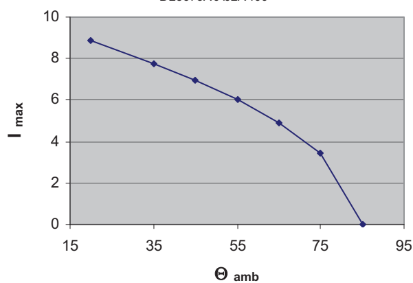
Max. allowable current (rms) at specific ambient Temp. B25673A0102A400
