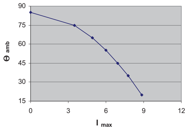
Max. allowable ambient Temp. at specific current (rms) B25673A0102A400
